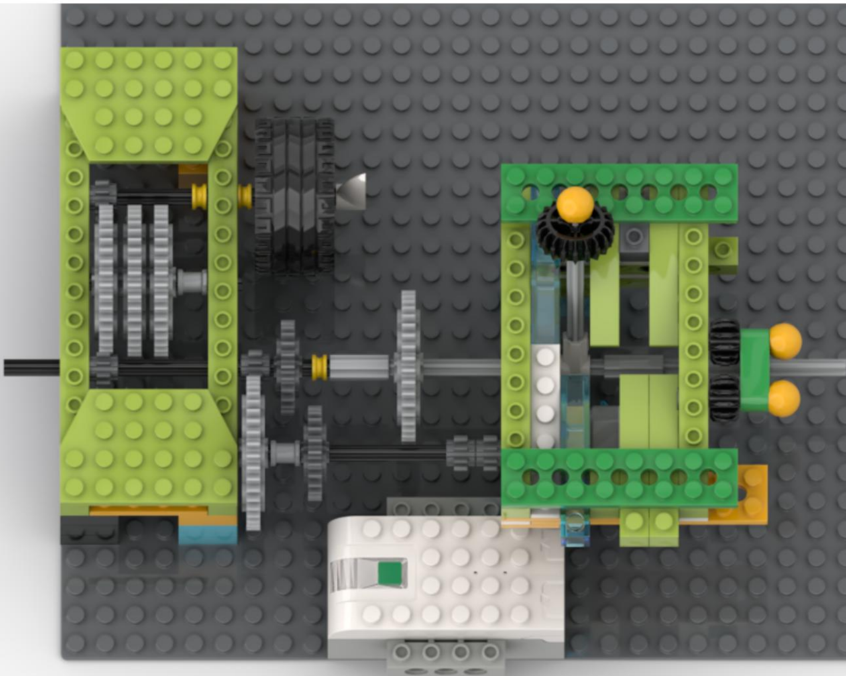
3 speeds gearbox
